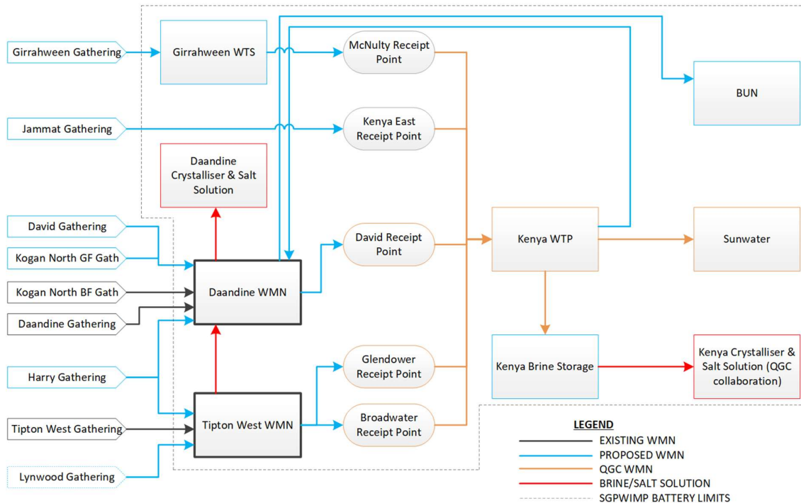
Figure 4-2 Proposed SGP CSG Water Management Network
