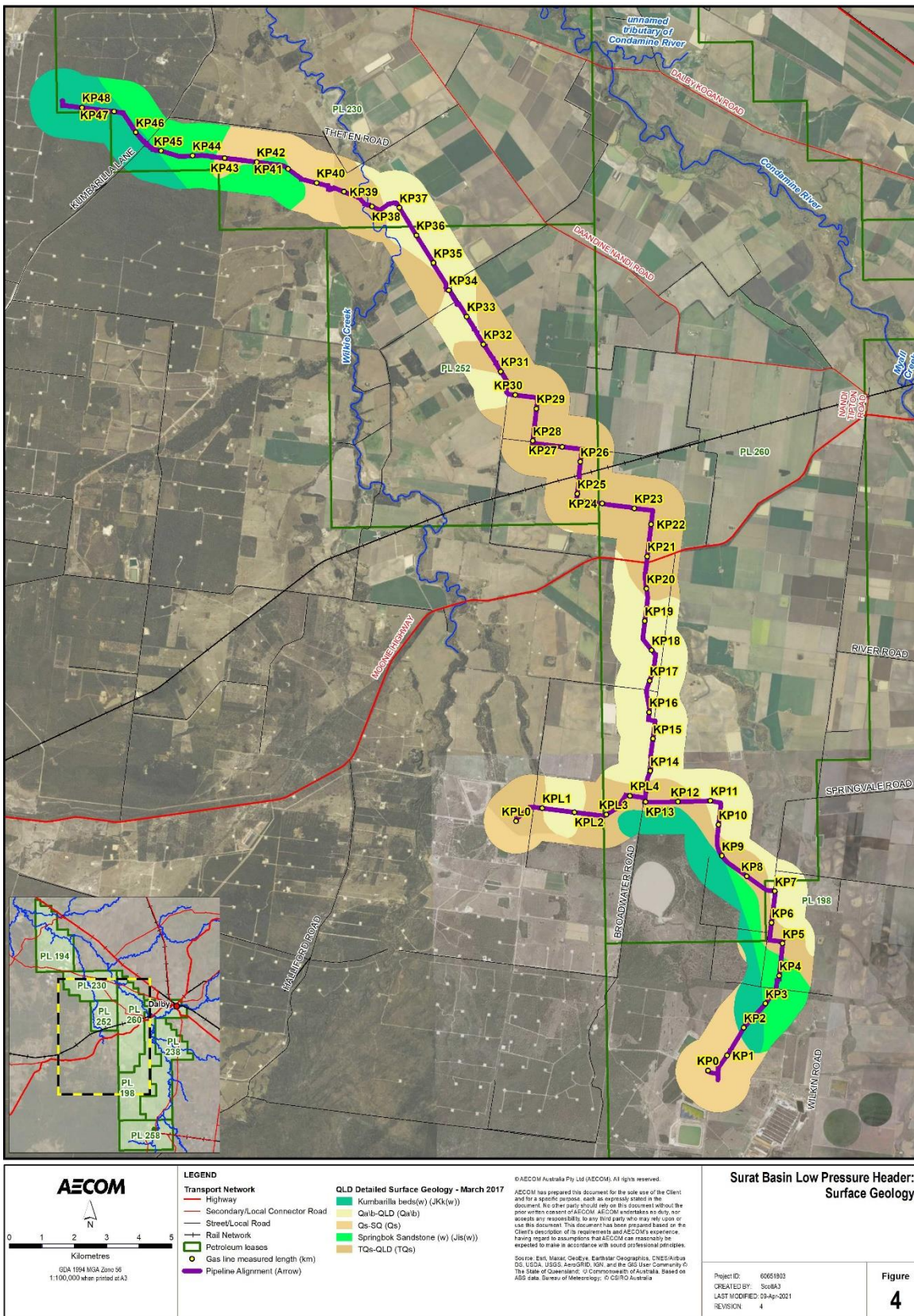
Figure 4 Surface Geology
