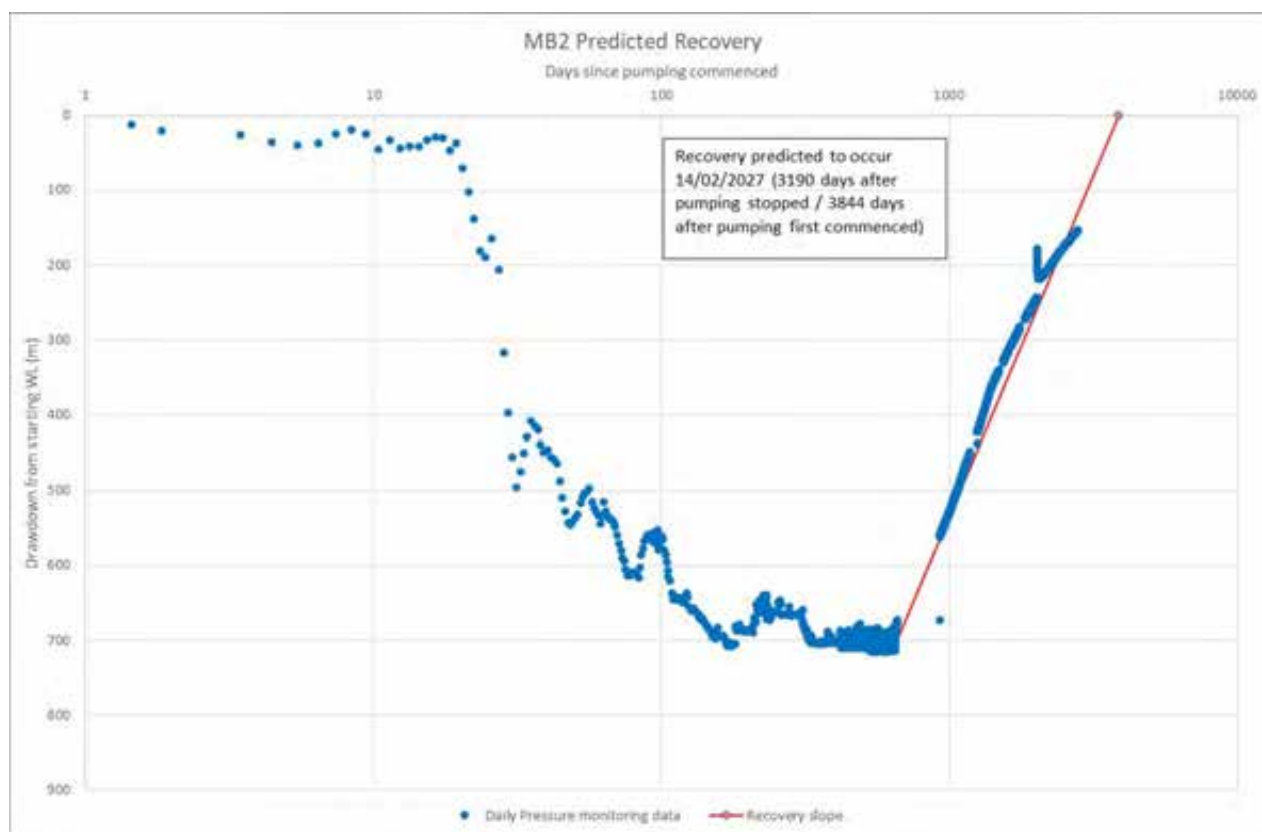
Figure 7: MB2 recovery data
