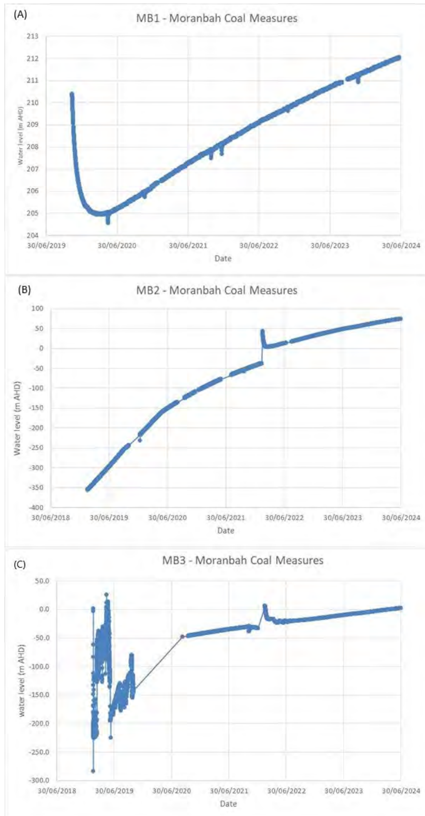
Figure 9: Deep bores with a long-term recovery of water level
