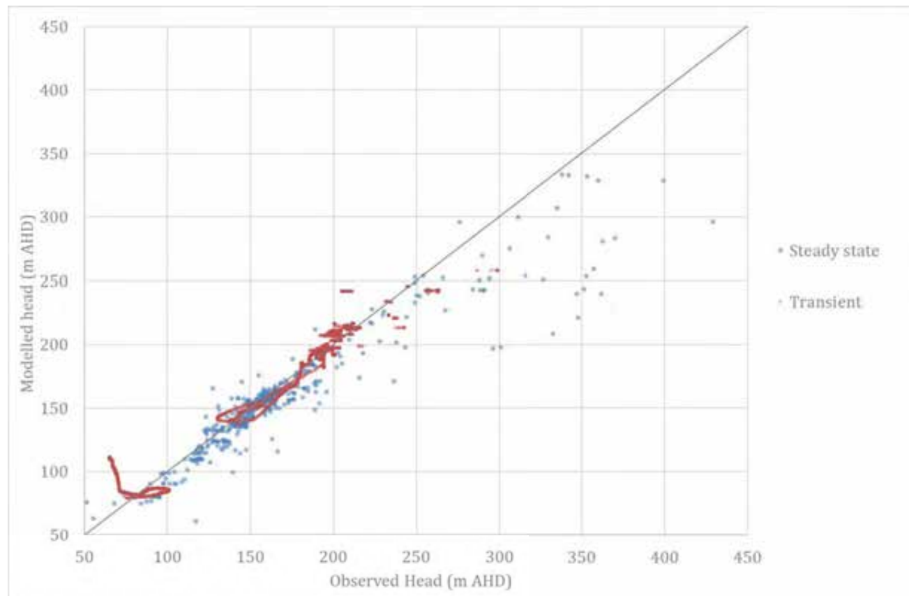
Figure 25: Measured vs. Simulated Groundwater Levels - 2025 Bowen UWIR model
