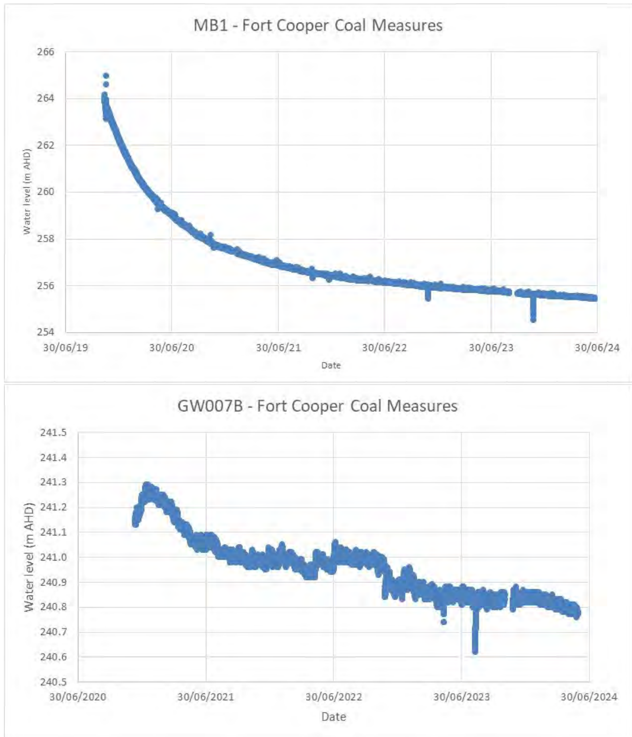
Figure 10: Deep bores with a long-term declining water level
