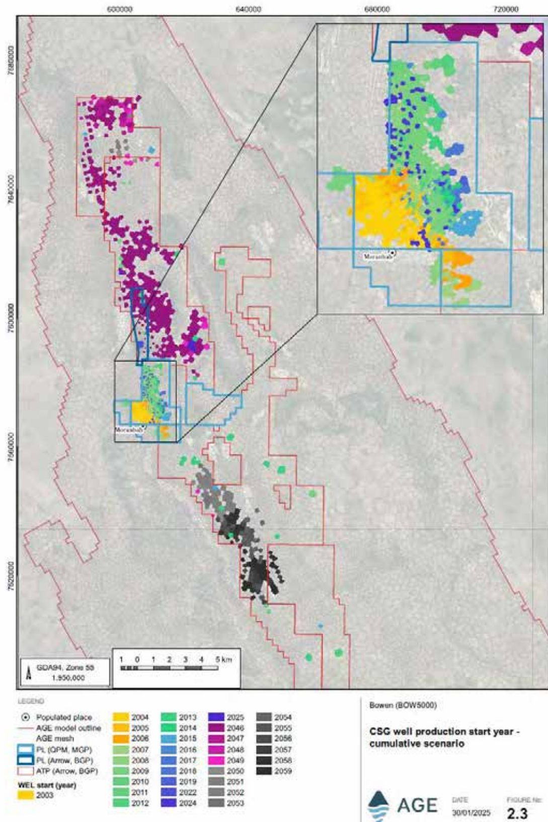
Figure 21: CSG Well Production Start Year – Cumulative Scenario
