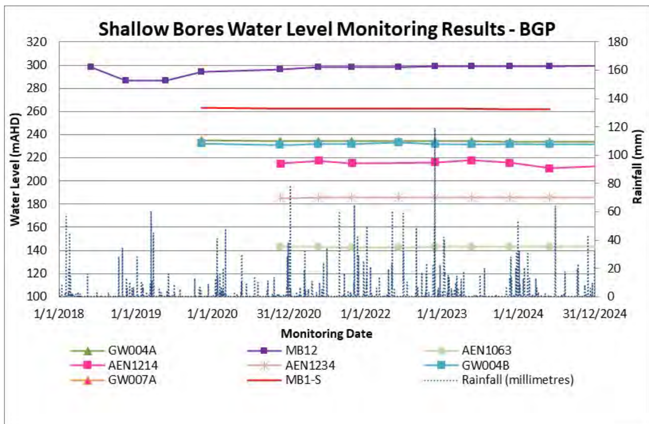
Figure 4: BGP shallow bores water level monitoring results
