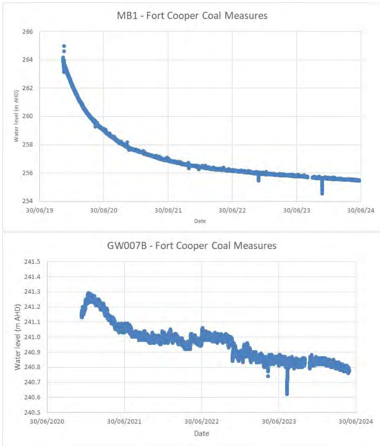
Figure 13: Deep Bores with a Long-term Declining Water Level
