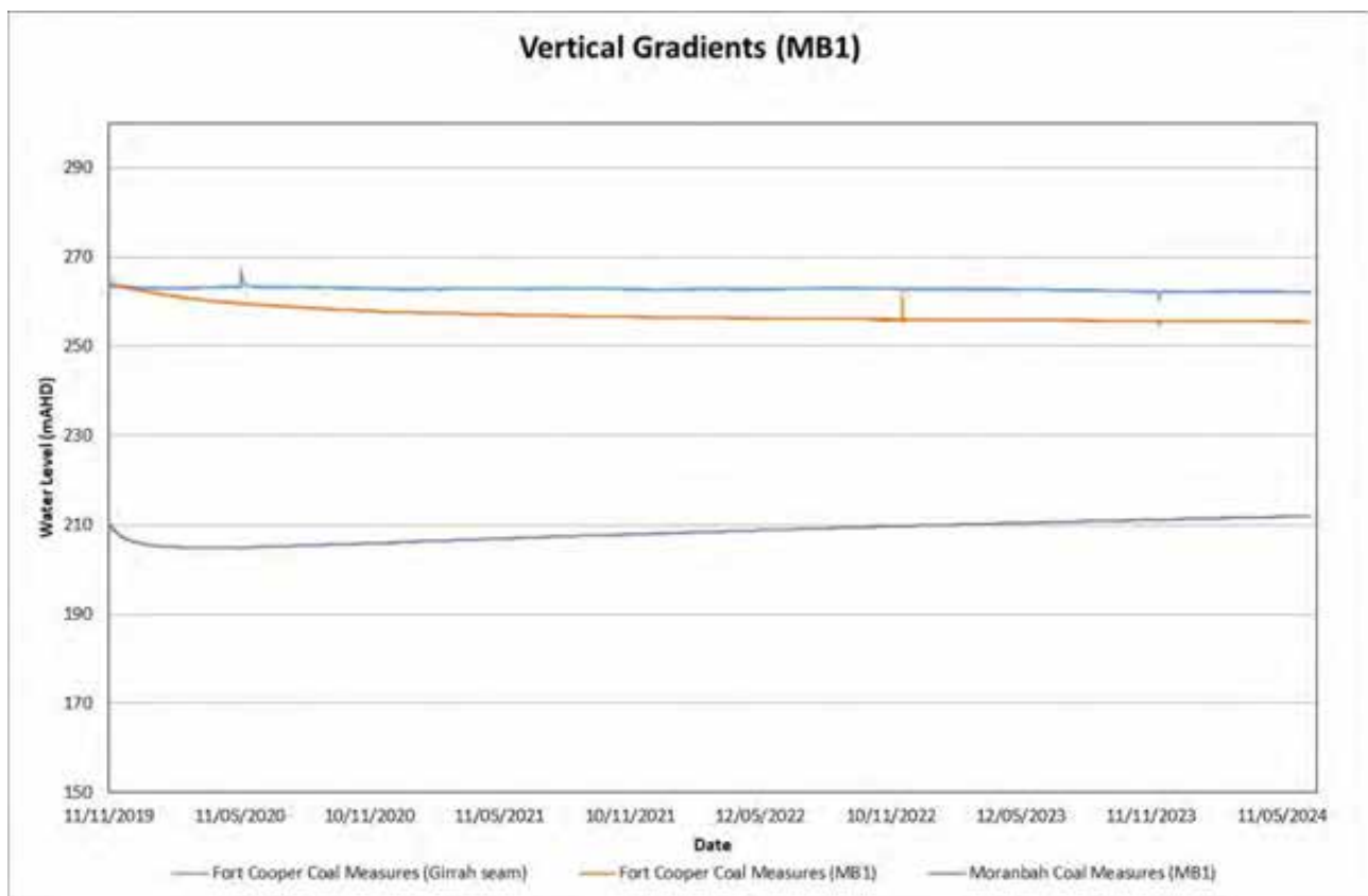
Figure 11: Review of vertical gradients for MB1
